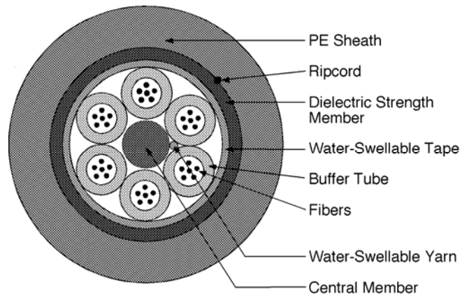
Figure 05-1 Dielectric OSP Fiber Optic Cable
