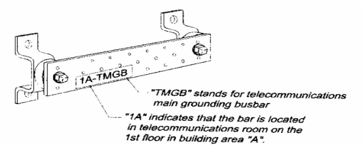
Figure 08-1 TMGB/TGB Busbar Labeling
