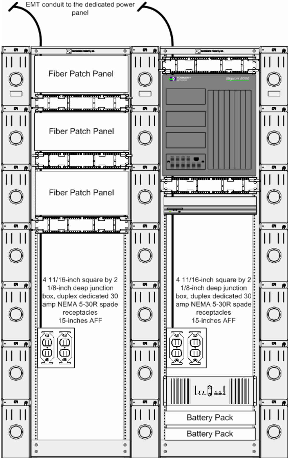
Figure 07-1 Typical ADF Equipment
