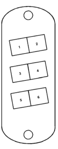
Figure 09-2 Vertical 568SC Duplex Fiber Optic Connector Panel Numbering Sequence
