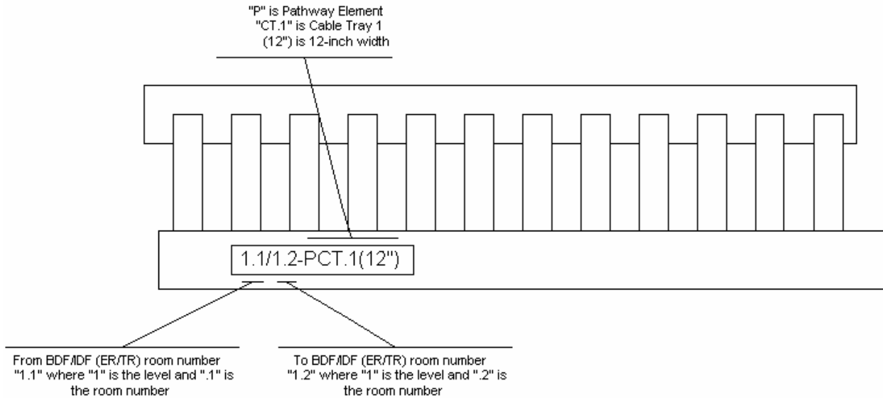
Figure 4-5 Cable Tray Labeling
