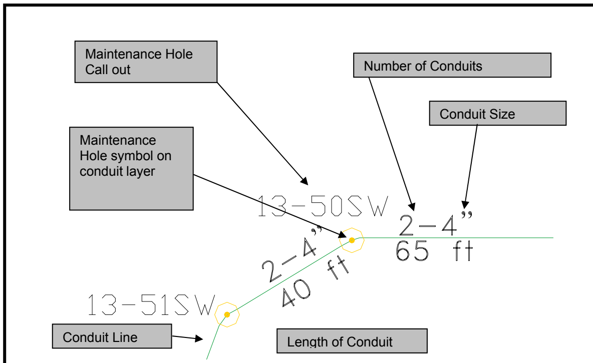
Figure 12-6 OSP Drawing Maintenance/Hand Hole and Conduit Callouts
