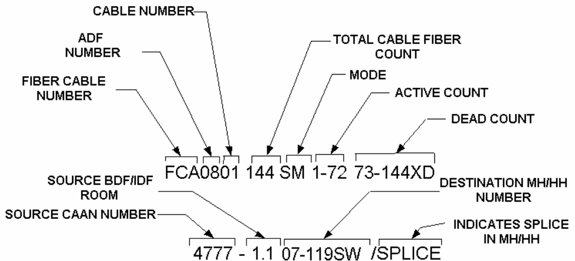
Figure 12-4 OSP Drawing MH/HH Fiber Optic Cable Callout
