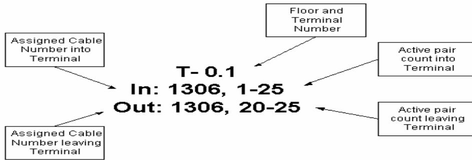
Figure 12-5 OSP Drawing Terminal Callouts
