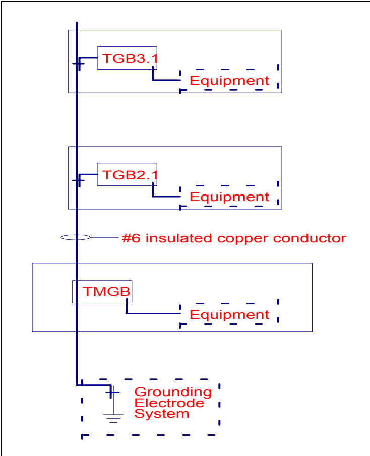
Figure 08-2 Bonding and Grounding Layout
