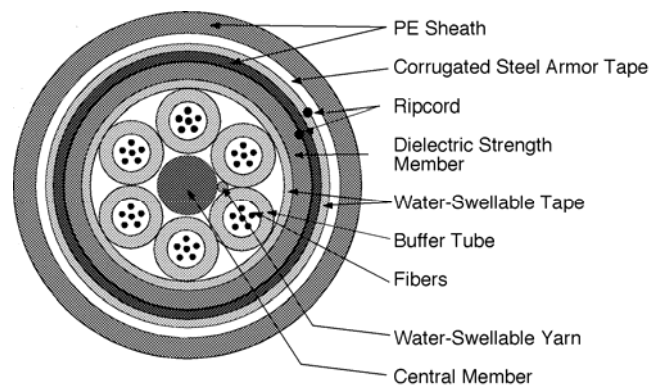
Figure 05-2 Armored OSP Fiber Optic Cable
