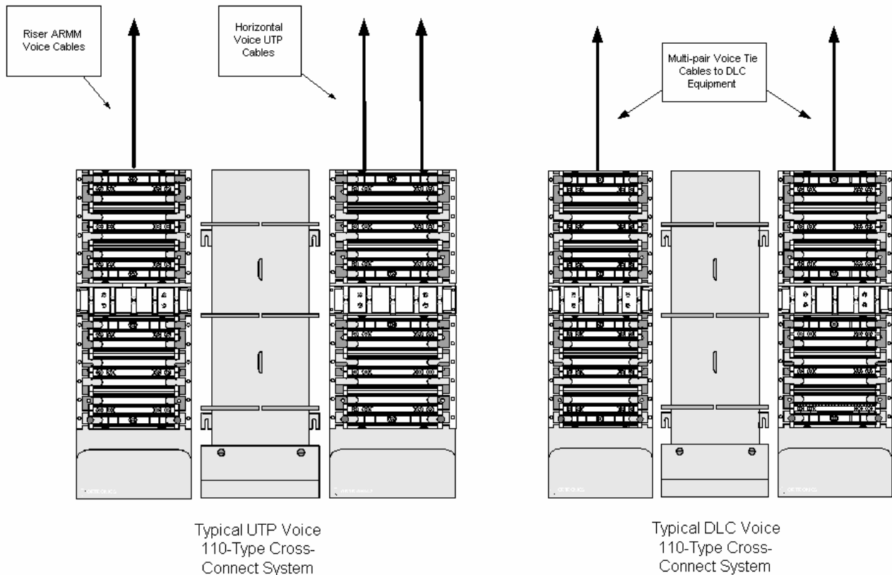
Figure 6-2 Voice 110-type Cross-Connect System
