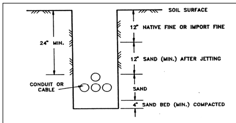
Figure 7-2 Trench cross-section for non-paved areas.
