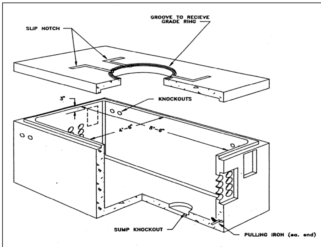
Figure 2-1 Typical Maintenance Hole
