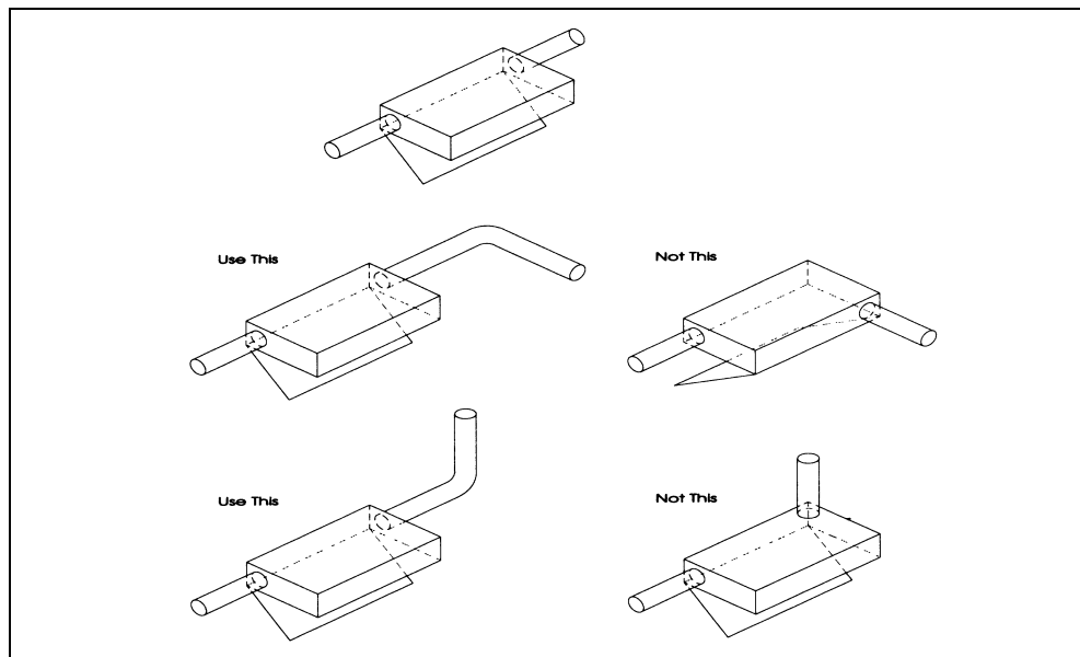
Figure 4-6 Pull Box configurations
