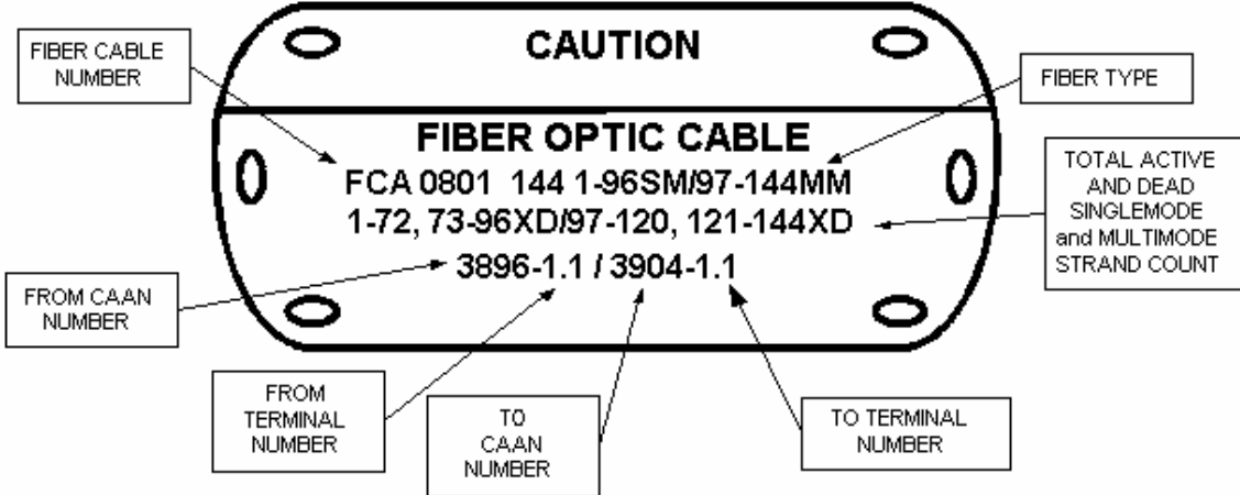
Figure 09-6 Fiber Optic Cable Label Sequence (MH/HH Splice)
