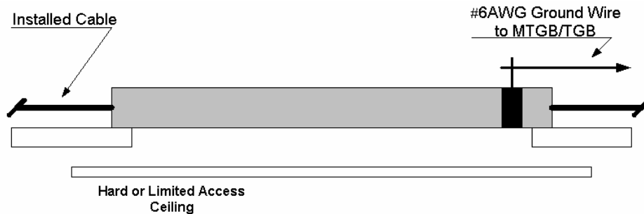
Figure 4-4 EMT Conduits Placed Above Hard or Limited Access Ceiling
