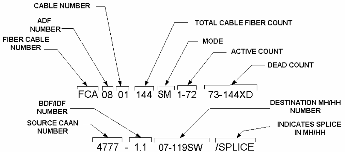
Figure 12-3 OSP Drawing CAA Fiber Optic Cable Callout
