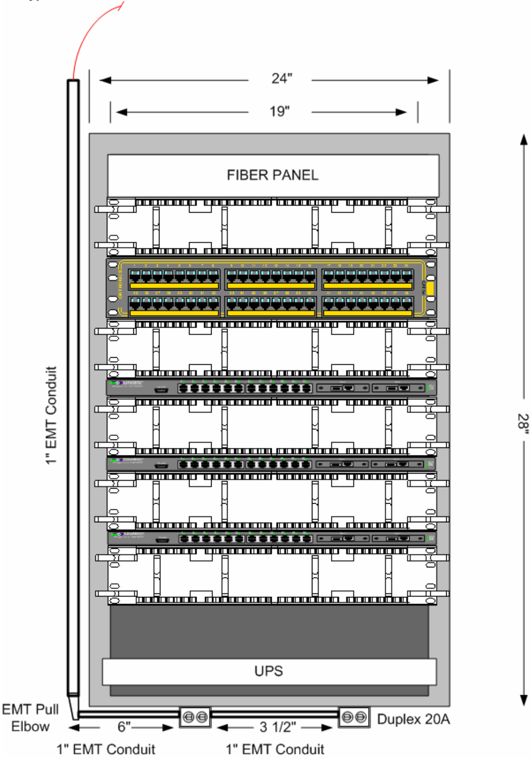
Figure 07-7 Type 3 IDF Wall Mounted Cabinet:
