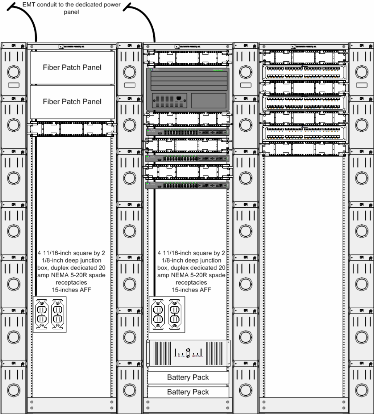
Figure 07-3 BDF/IDF Equipment Racks:
