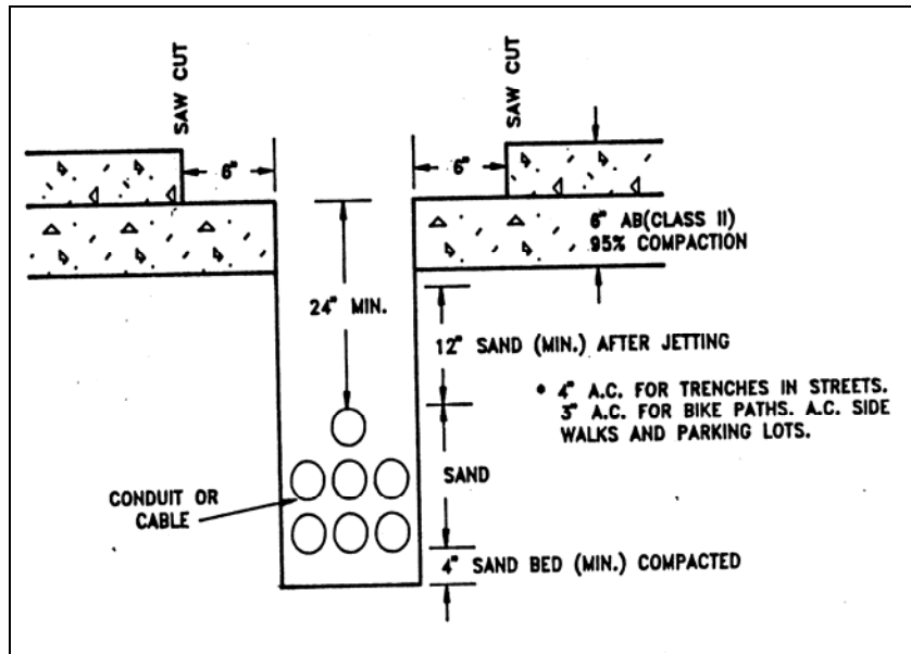
Figure 7-1 Trench cross-section for paved areas
