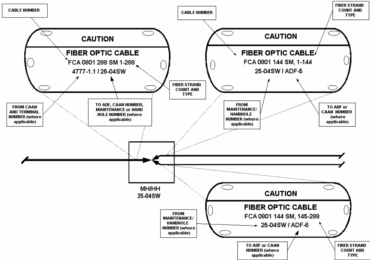
Figure 09-7 Building Entrance Terminal Label Sequence
